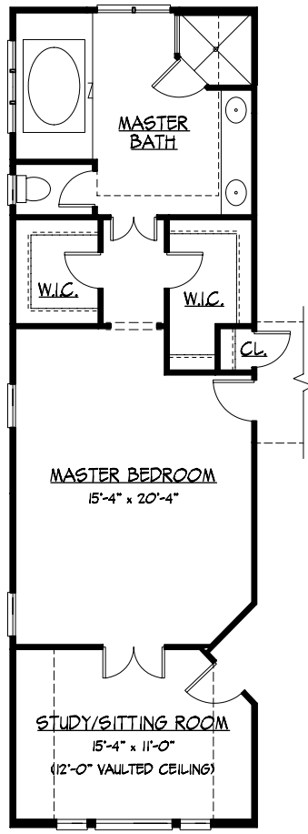
OPT. 5TH BEDROOM FIRST FLOOR PLAN
