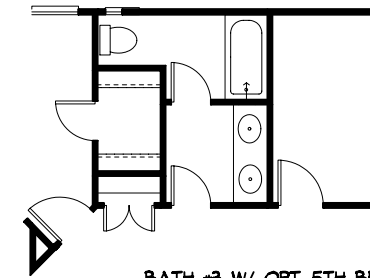
BATH #3 W/ OPT. 5TH BEDROOM SCALE: P:\mg\107\devonshire\second.flr 1/4" = 1'-0"
